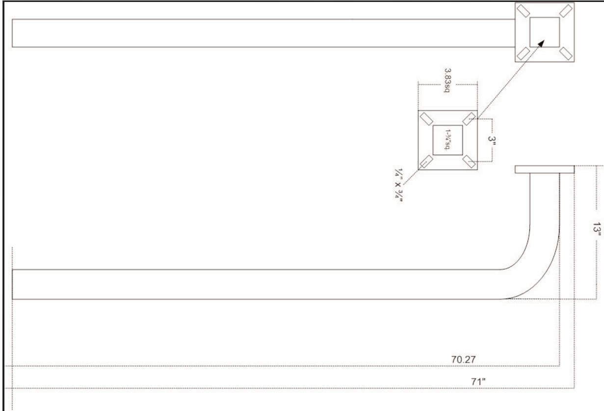
18-011 Direct burial Pedestal
